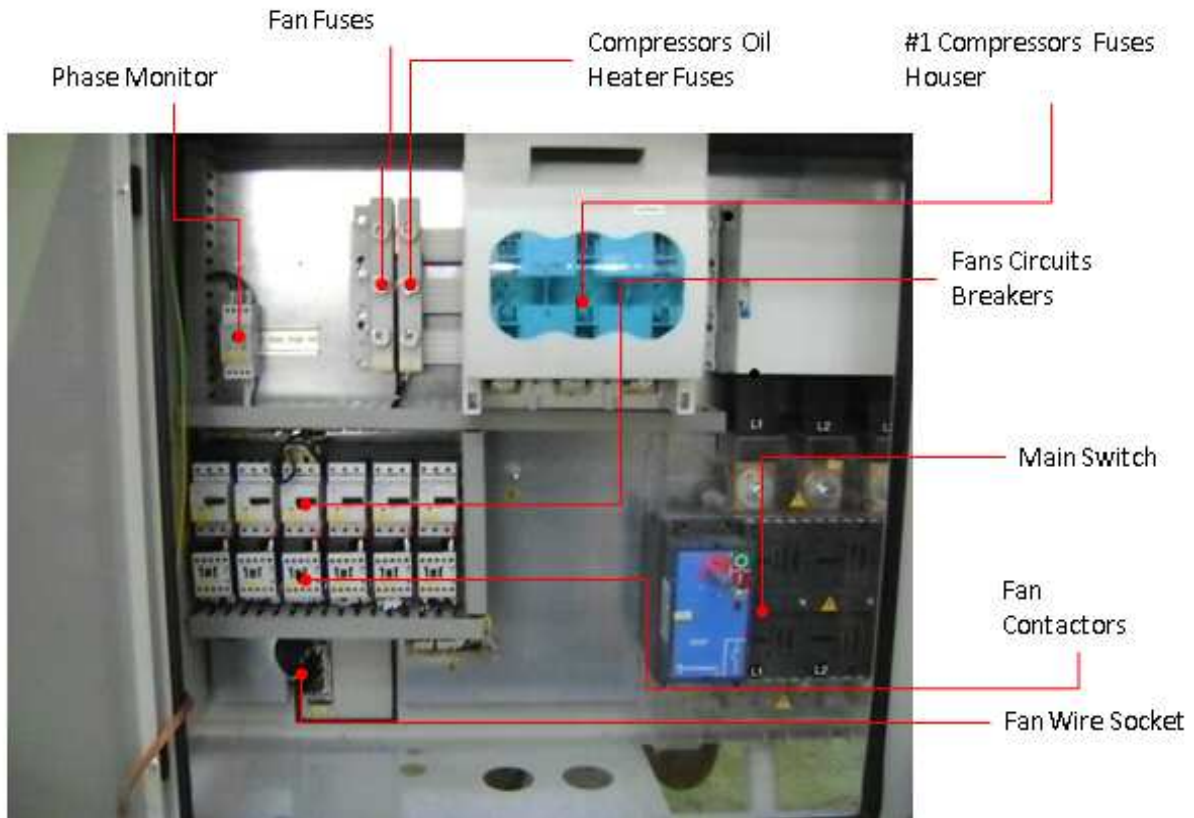
Figure 3, Power Panel, Right Side
