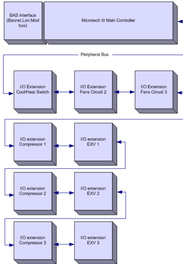
Figure 3, System Architecture
