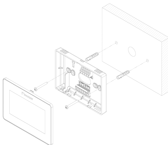
Figure 3 – Wall Mounting
