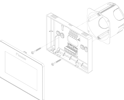
Figure 4 – Installation with 502 electric box
