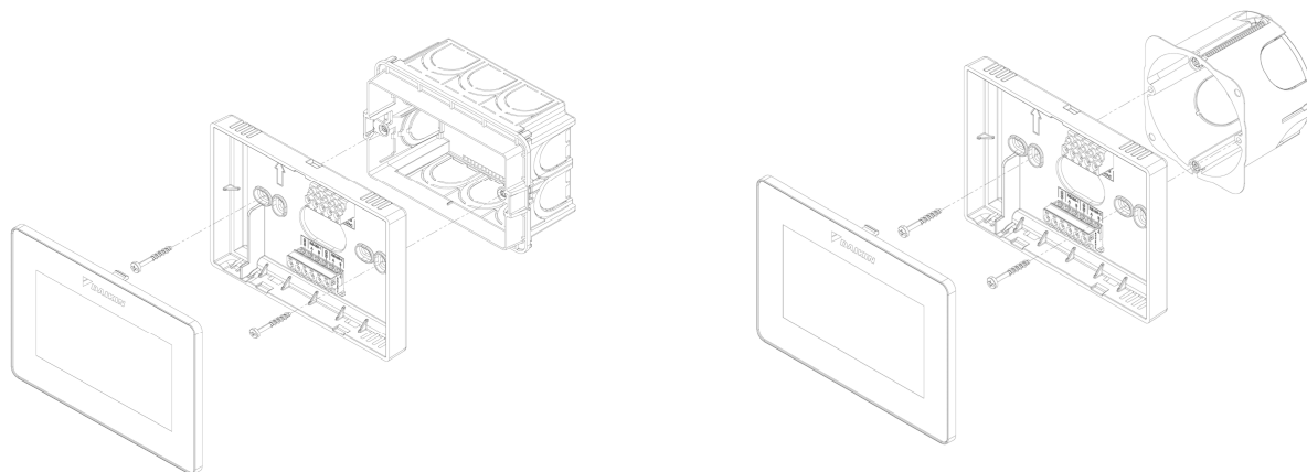
Figure 4 – Installation with 503 electric box
