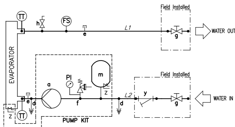
Figure 12 – Schéma hydraulique
