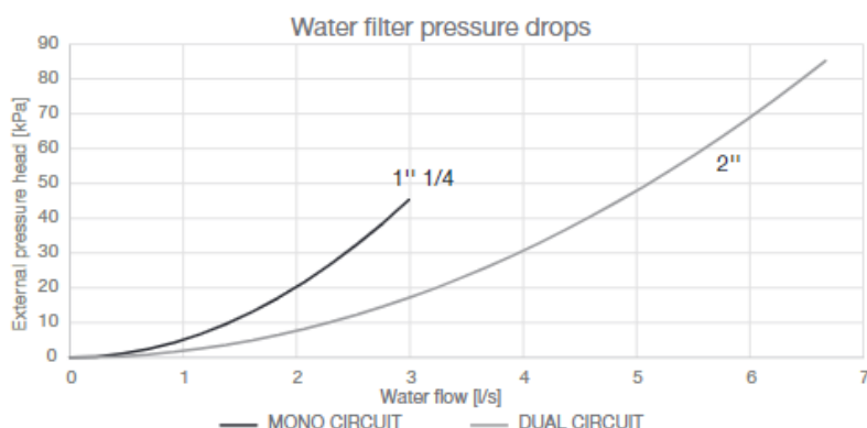
Рис. 12 - Water filter pressure drops
