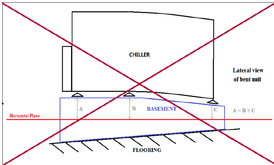
Fig. 22- Unit levelling
